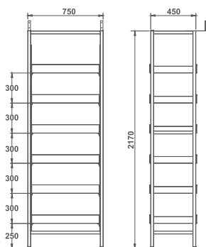
ESTANTE MODULAR WALK IN COOLER
