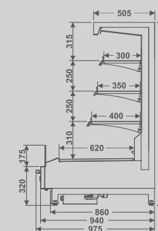
ESVVA Expositor Semi Vertical Vision Alto
